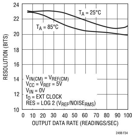
Figure 34. Resolution ( N_{\text{RMS}} \leq 1\text{LSB} ) vs Output Data Rate and Temperature
